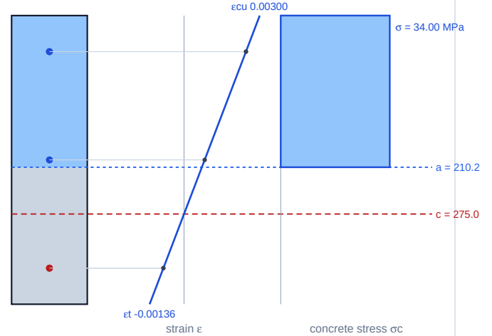
Longitudinal section — strain and stress over the depth D\theta=400
